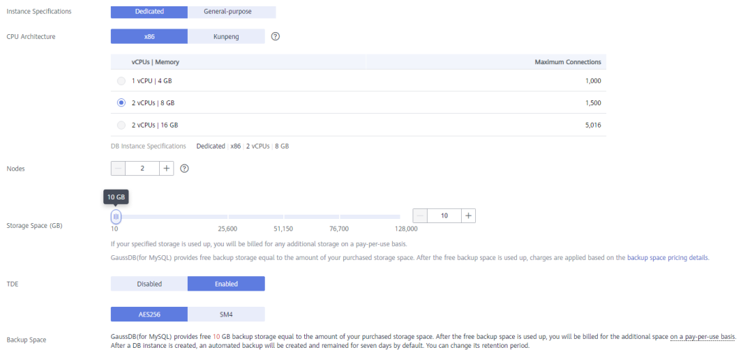
Figure 2-6 Specifications and storage of a yearly/monthly DB instance
